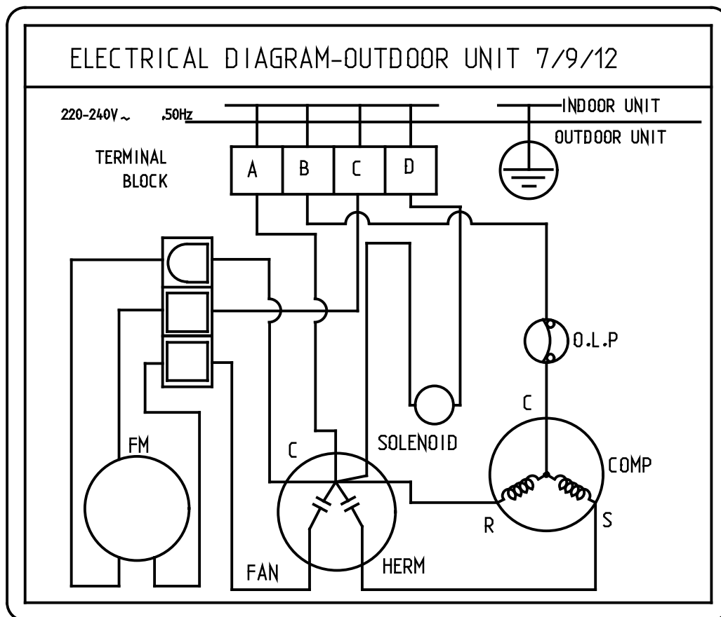
CIRCUIT DIAGRAM OUTDOOR UNIT 7/9/12K
