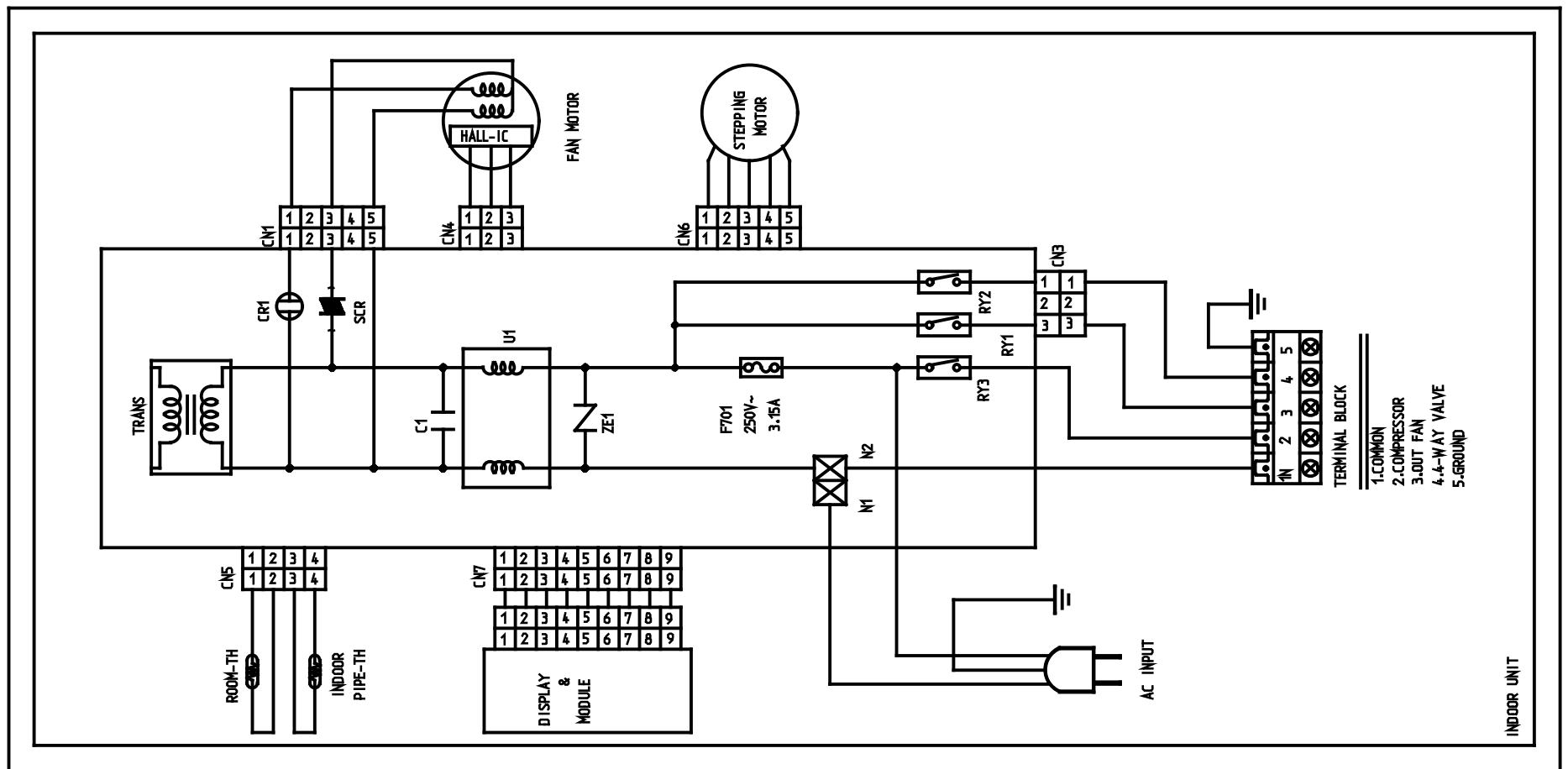
CIRCUIT DIAGRAM INDOOR UNIT 7/9/12K
